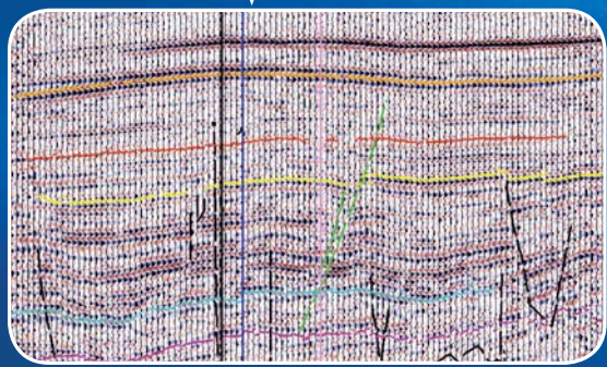
Seismic interpretation
